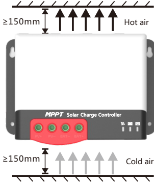
Figure 2.1 Installation and Heat Dissipation
