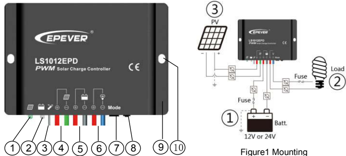
Figure1 Mounting
